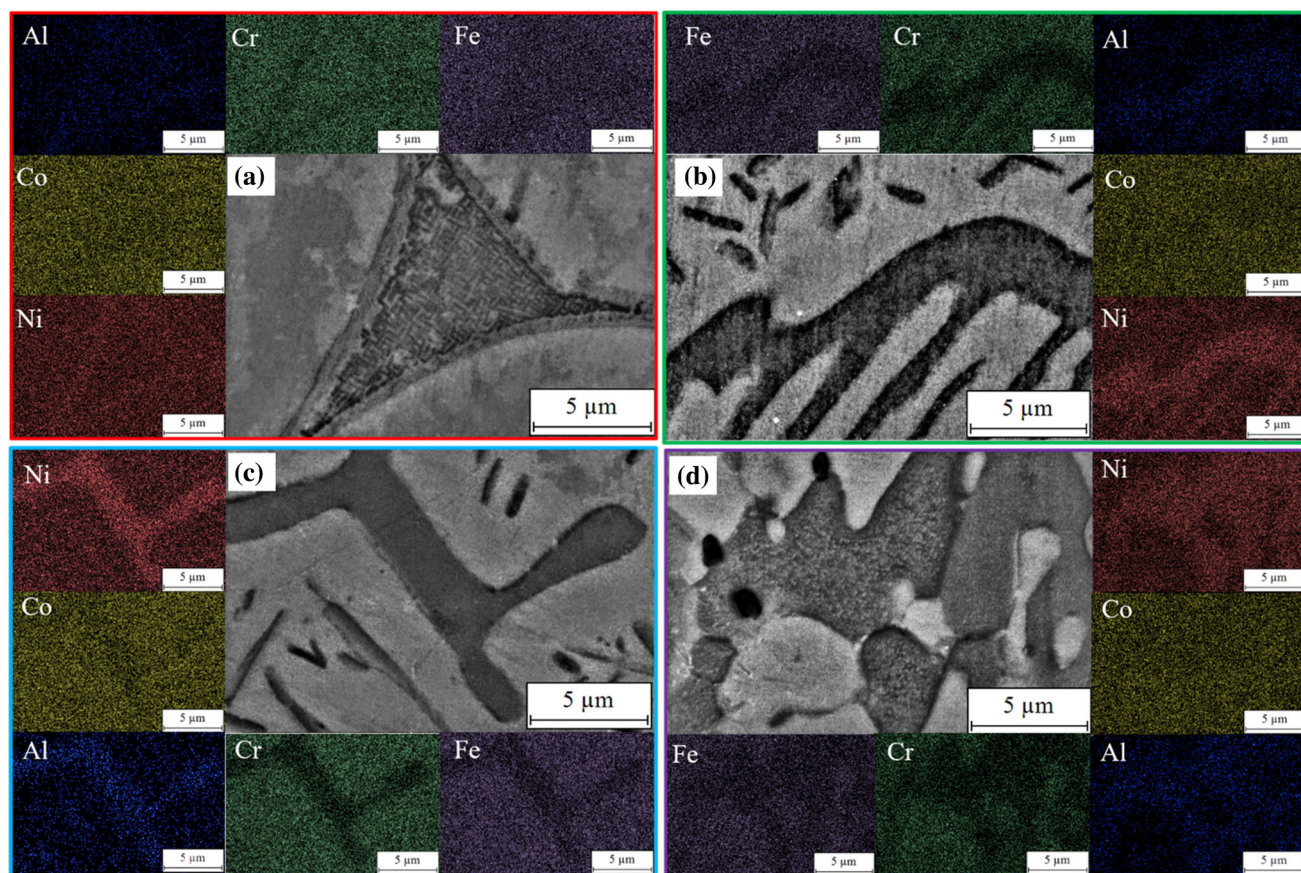
Fig. 6 BSE images and EDS maps of \text{Al}_{0.5}\text{CoCrFeNi} alloy: (a) as-cast, (b) homogenized at 1100 °C for 24 h, (c) cold-rolled by 60%, (d) annealed at 1100 °C for 1 h
