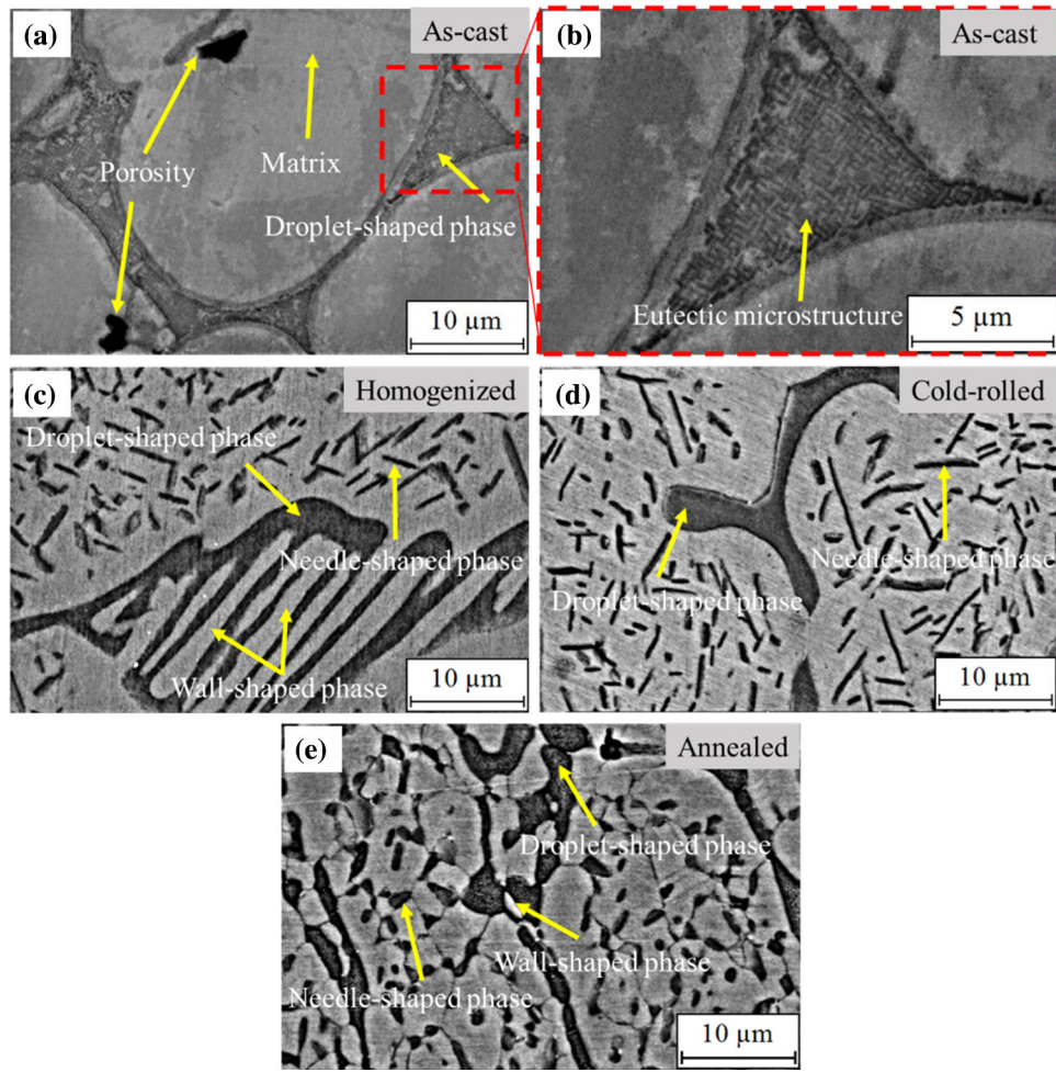
Fig. 5 SEM images, related to the microstructure of \text{Al}_{0.5}\text{CoCrFeNi} alloy: (a) as-cast, (b) magnified of the interdendritic region in the as-cast state showing a eutectic microstructure, (c) homogenized at 1100 °C for 24 h, (d) cold-rolled by 60%, (e) annealed at 1100 °C for 1 h
