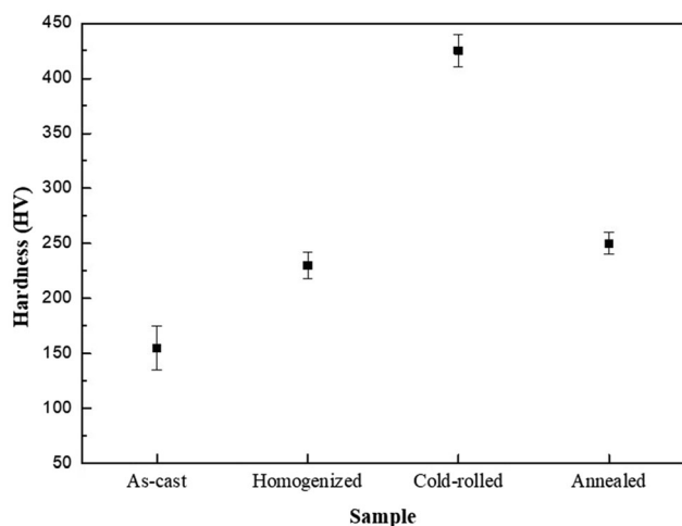
Fig. 7 The hardness of \text{Al}_{0.5}\text{CoCrFeNi} alloy in different conditions
