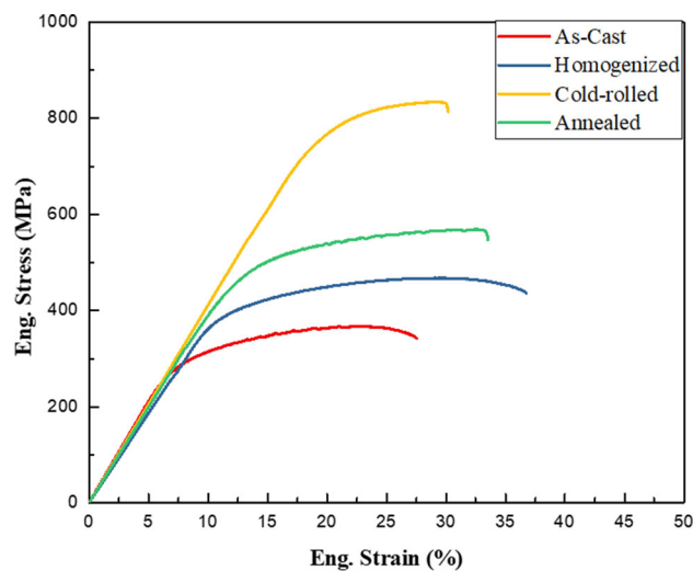
Fig. 8 Engineering tensile curves of \text{Al}_{0.5}\text{CoCrFeNi} HEA in different conditions
