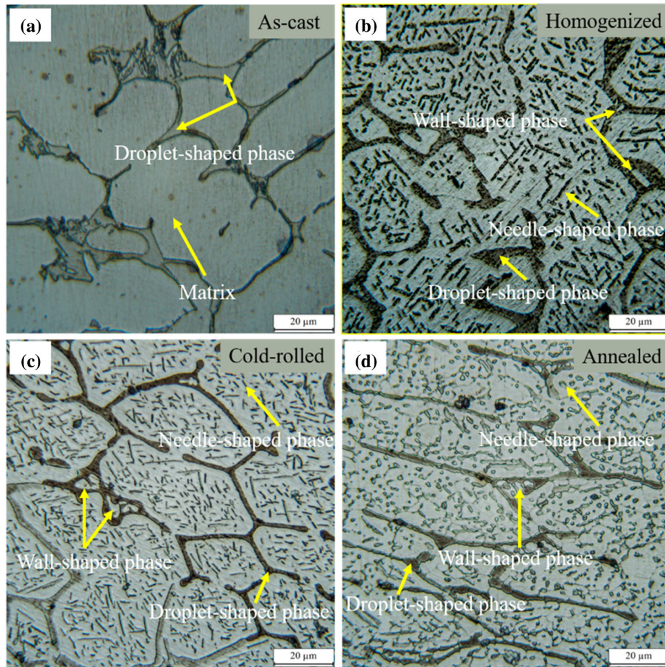
Fig. 4 Optical micrographs, related to the microstructure of \text{Al}_{0.5}\text{CoCrFeNi} alloy: (a) as-cast, (b) homogenized at 1100\text{ }^{\circ}\text{C} for 24 h, (c) cold-rolled by 60%, (d) annealed at 1100\text{ }^{\circ}\text{C} for 1 h
